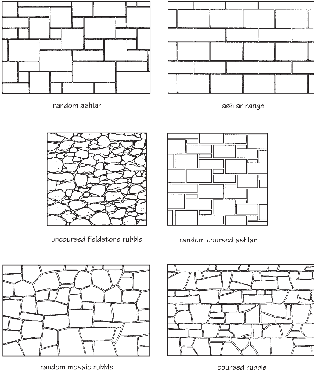
Figure 5-7 Stone bonding patterns. (From Ramsey and Sleeper, Architectural Graphic Standards , 6th edition, ed., 1970. Reprinted by permission of John Wiley & Sons, Inc., and Allen, Fundamentals of Building Construction , 3rd ed., 1999.)
